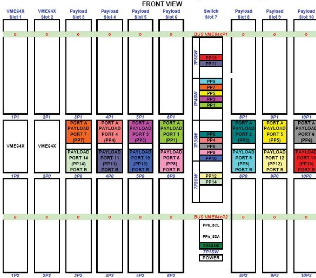
VXS BACKPLANE 10 SLOTS, 6U, Single-Star (1SW+7PP+2VME64X)
